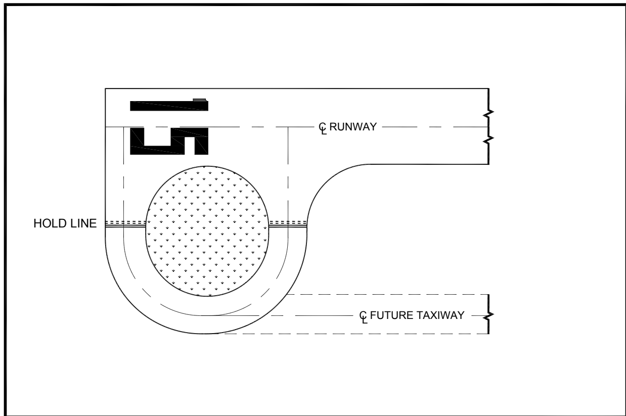
Figure 4-29. Taxiway turnaround
