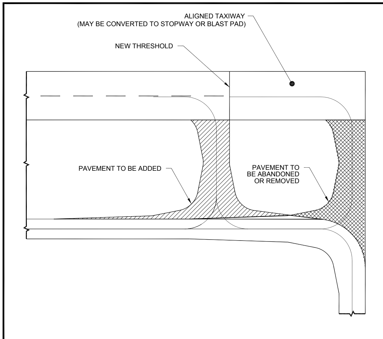
Figure 4-32. Aligned taxiway
